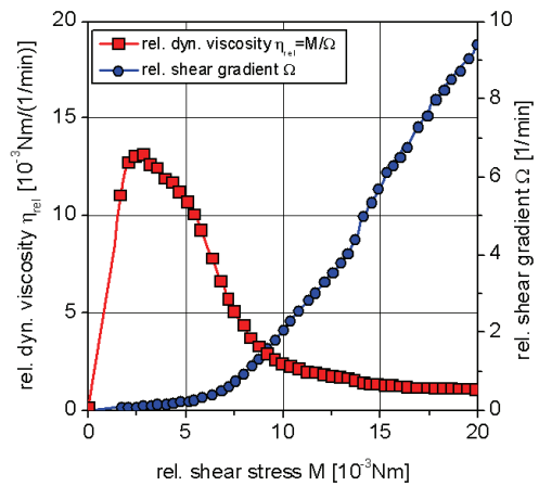
Figure 3. Determination of the relative yield stress \tau_{0rel} from the maximum of the relative viscosity curve, measured using a CS-ramp.
