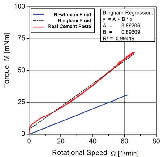
Figure 1. Flow curves of a Newtonian Fluid, an ideal Bingham-material and a real paste.
