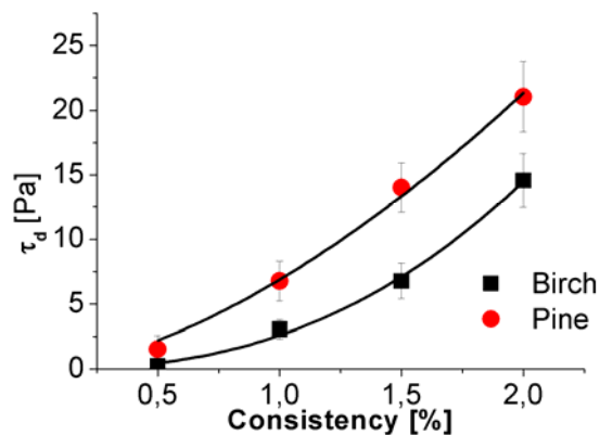
Figure 7. The disruptive shear stress \tau_d as a function of consistency for pine and birch fiber suspensions. The solid lines give the fitted values according to Eq. 3.
