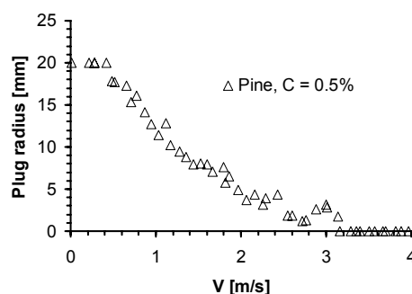
Figure 6. The measured fiber plug radius as a function of flow velocity for pine at consistency 0.5 %.
