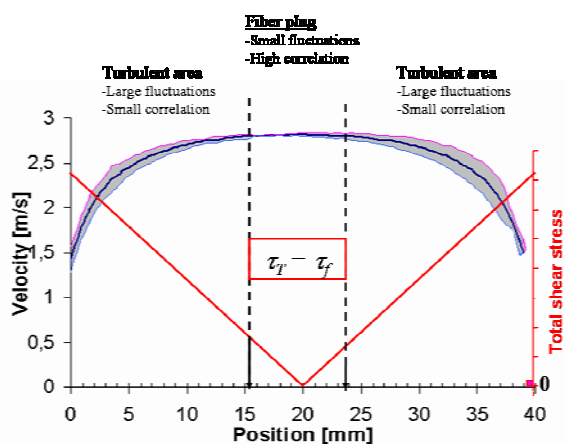
Figure 3. The averaged velocity profile (solid line) and the velocity fluctuations (grey area) of fiber suspension (birch, consistency 1%). The position of the fiber plug core is also shown. \tau_f indicates the shear stress of the fiber phase.
