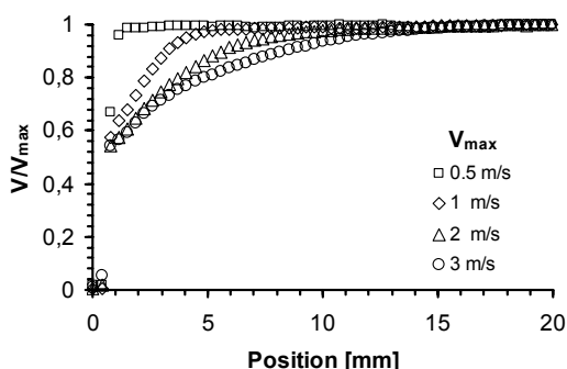
Figure 4. Averaged velocity profiles of fiber suspension (pine at consistency 0.5% by weight) for several flow rates measured by the pulsed ultrasound Doppler velocimeter. The diameter of the tube is 40 mm. The velocity values are scaled by the maximum velocity of each profile.
