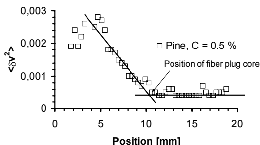
Figure 5. Turbulent intensity, as measured by PUDV, as a function of distance from the tube wall. The crossing point of two fitted solid lines indicates the position of the surface of fiber plug core.
