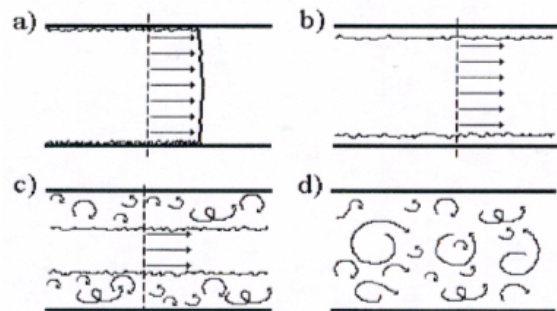
Figure 1. Flow regimes of fiber suspensions. (a) Plug flow regime. (b) Plug flow regime with lubrication layer. (c) Transient or mixed flow regime. (d) Turbulent flow regime. (The figure is reprinted from Modelling the Flow of Pulp Suspensions in Pipes , Bertel Myreen, Jaakko Pöyry Oy.)
