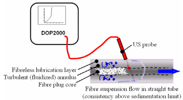
Figure 2. The pulsed ultrasound Doppler velocimeter (Signal Processing-DOP2000).
