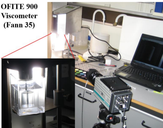
PIV - camera NanoSense MKIII-plus (Dantecdynamics)
